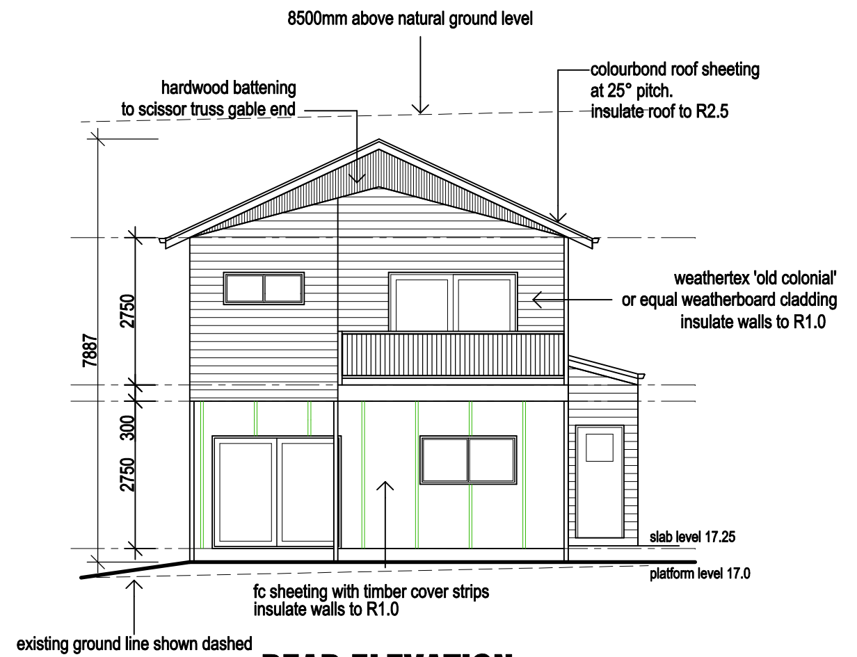
REAR ELEVATION
